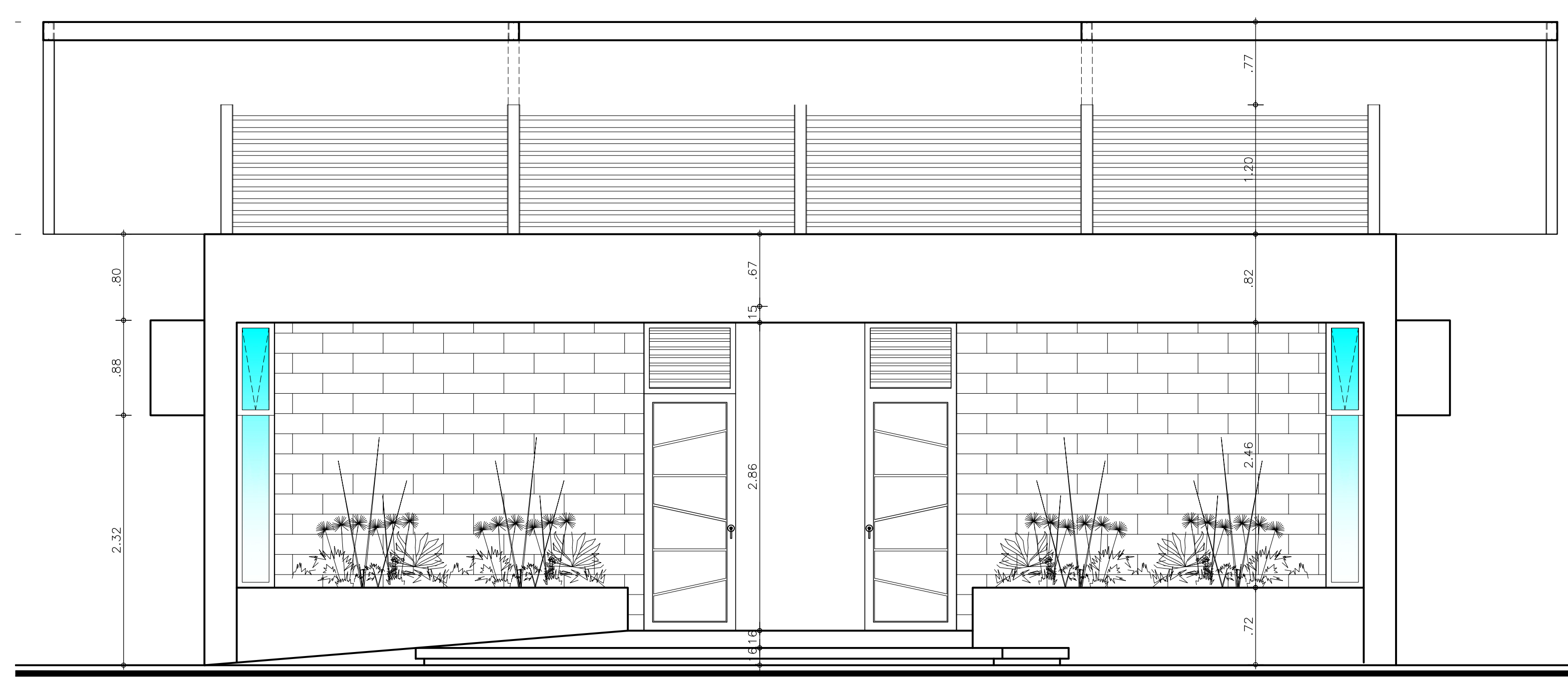
FACHADA PRINCIPAL ESC: 1: 50
